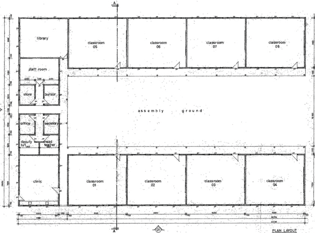
PLAN LAYOUT
